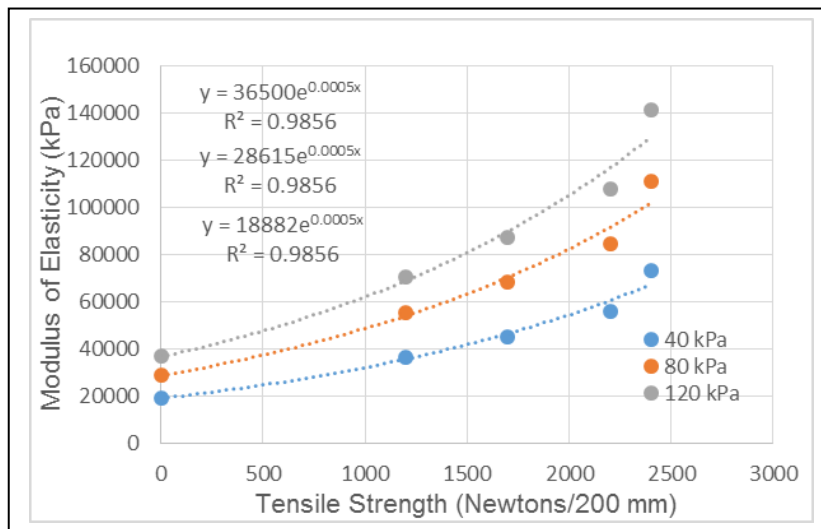
Fig. 4: Variation of Modulus of Elasticity with geotextile tensile strength of Terram
