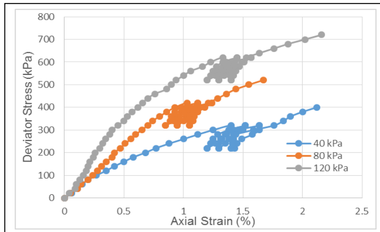
Fig. 2: Stress-strain behaviour of saturated LBS specimens confined by T1000 under three different cell pressures.
