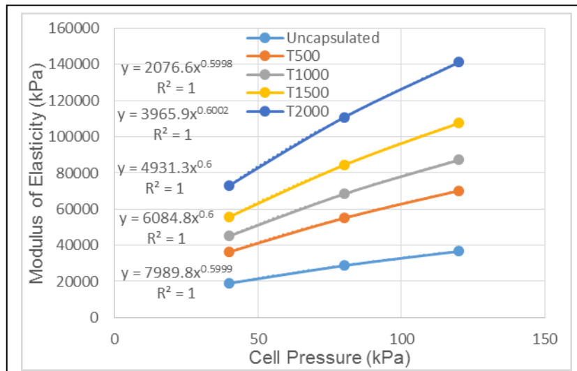
Fig. 6: Variation of Modulus of Elasticity of the composite with triaxial cell pressure
