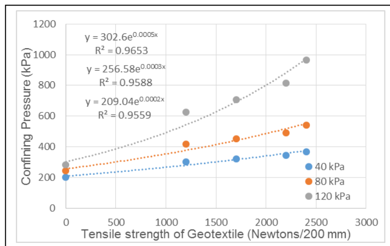
Fig. 5: Variation of surrounding confining pressure with geotextile tensile strength of Terram
