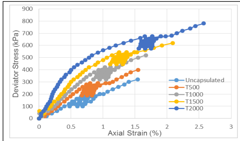
Fig. 1: Stress-strain behaviour of saturated LBS specimens confined and not confined by 'Terram' (cell pressure = 80 kPa)
