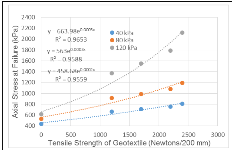
Fig. 3: Variation of axial stress at failure with geotextile tensile strength of Terram
