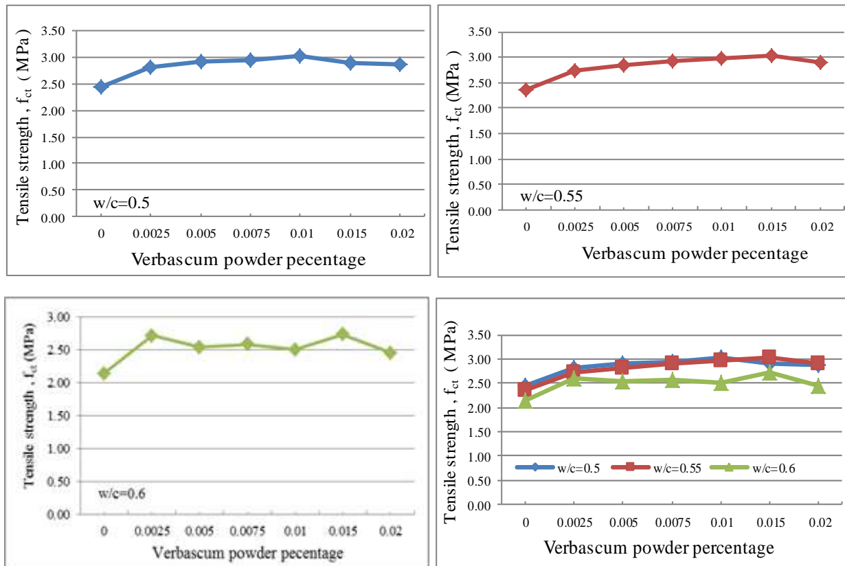
Fig. 2: Tensile strength of concrete samples containing Verbascum powder.
