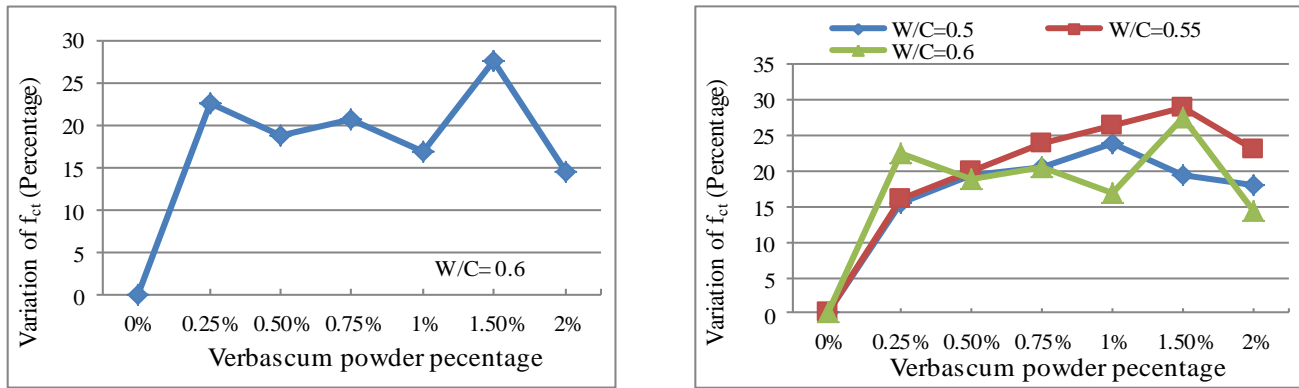
Fig. 3: Changes of tensile strength of concrete containing Verbascum powder.
