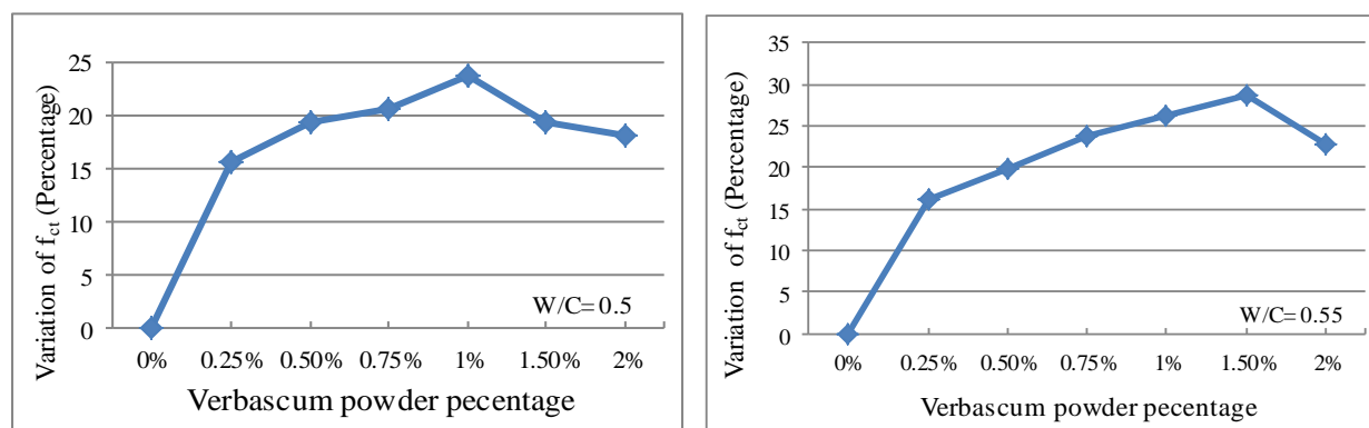
Fig. 2: Tensile strength of concrete samples containing Verbascum powder.
